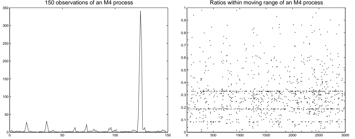
Figure 3: A demo of multiple signature patterns. Left figure is a time series plot of 150 observations of process Y_{td} = \max_{1 \leq l \leq 3} \max(a_{l1d}Z_{l,t-1}, a_{l0d}Z_{lt}, a_{l,-1,d}Z_{l,t+1}) for some d . Right figure is a time series plot of ratios Y_{td}/(Y_{td} + Y_{t+1,d} + Y_{t+2,d}) of 3000 observations.
