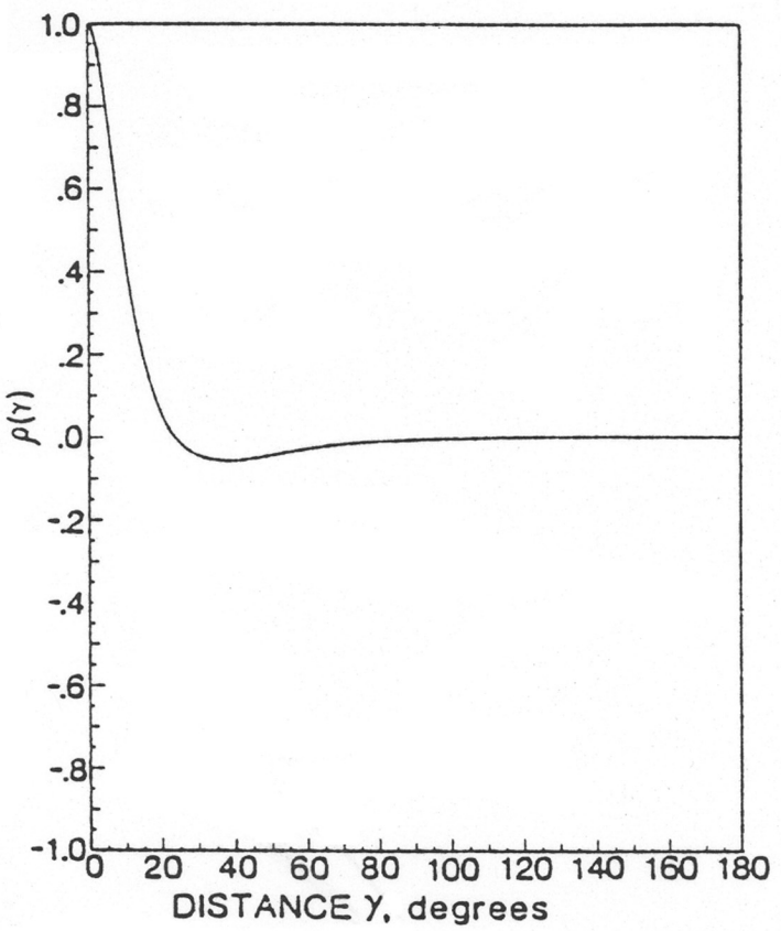
Figure 3: Correlation function for the ( \lambda_l ) of fig. 2.
