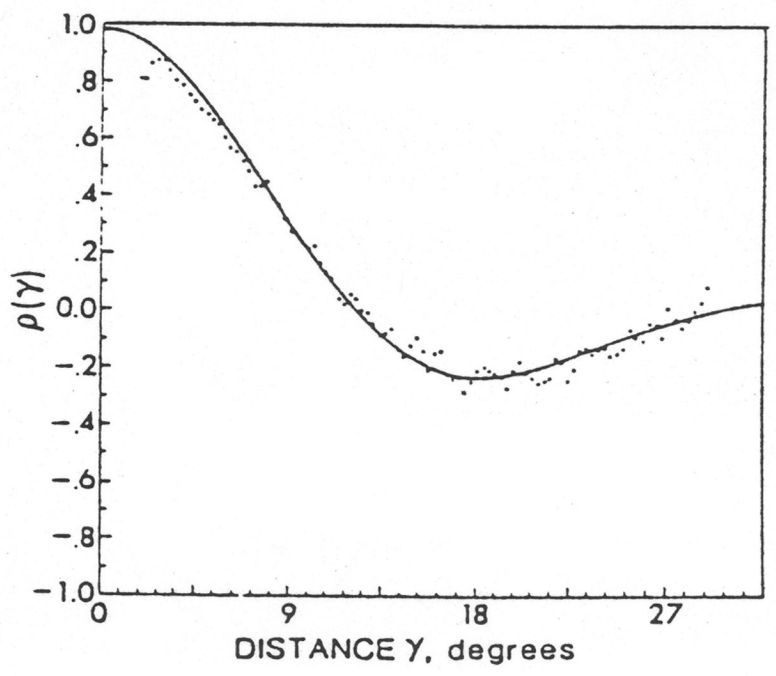
Figure 4: Sample Correlation Function.
