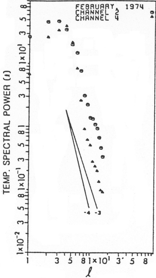
Figure 1: Temperature Spectral Power ( l ).
