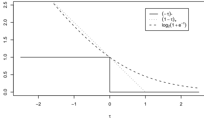
Figure 1: Comparison of (-\tau)_* , (1 - \tau)_+ and \log_2(1 + e^{-\tau}) .
