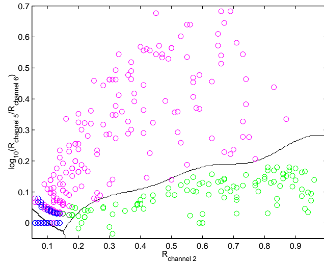
Figure 6: The classification boundaries determined by the MSVM using 370 training examples randomly selected from the bottom left plot in Figure 5.
