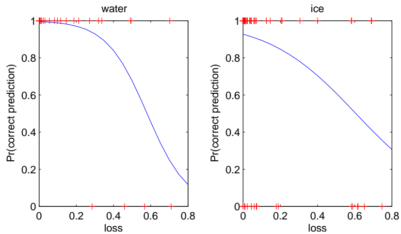
Figure 9: The estimated MSVM prediction accuracy as a function of the loss estimated via linear logistic regression, for the water and ice cloud predicted classes. Red ticks are the actual pairs of the hinge loss and the indicator of correct prediction (1:correct, 0:incorrect) for each test example.
