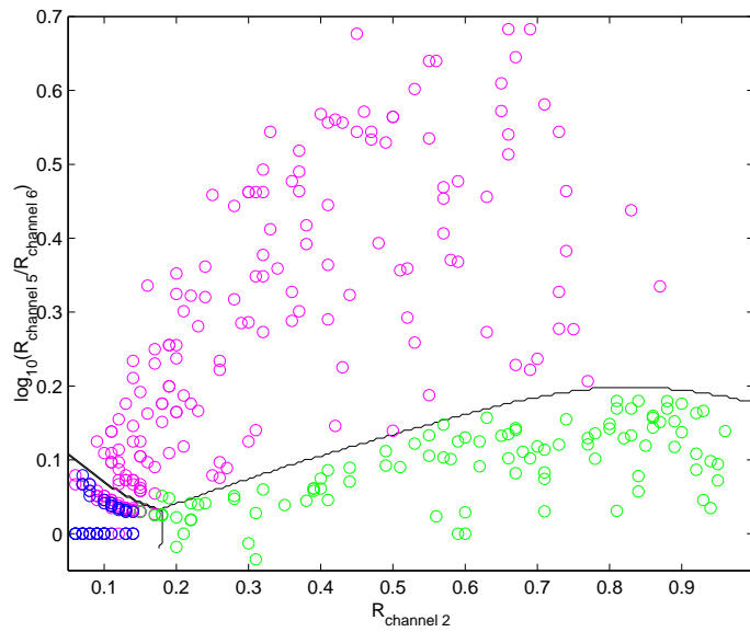
Figure 8: The classification boundaries determined by the nonstandard MSVM when the cost of misclassifying clear sky examples is four times as high as other types of misclassifications.
