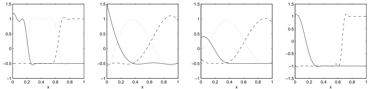
Figure 3: Left to Right: Optimum MSVM tuning, 5-fold cross validation tuning of the MSVM, GACV MSVM tuning, one-vs-many SVM.
