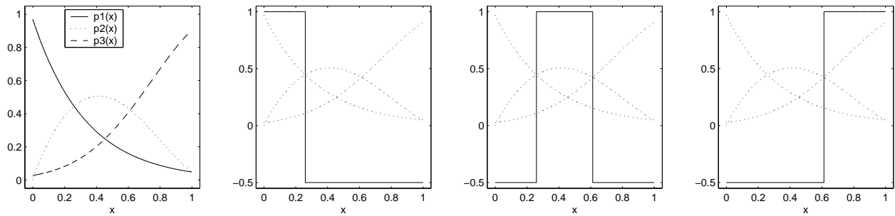
Figure 2: Probabilities and optimum f^j 's for three category SVM demonstration.
