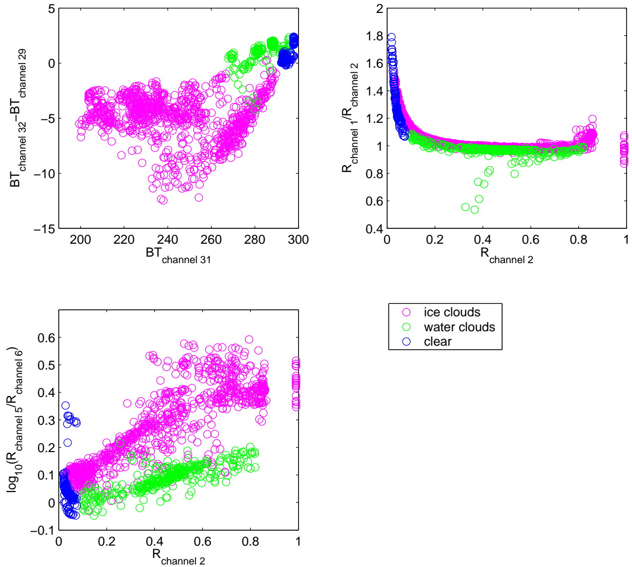
Figure 10: Scatterplots of BT_{channel31} vs BT_{channel32} - BT_{channel29} (top left), R_{channel1}/R_{channel2} vs R_{channel2} (top right), and R_{channel2} vs \log_{10}(R_{channel5}/R_{channel6}) (bottom left), labeled MODIS observations
