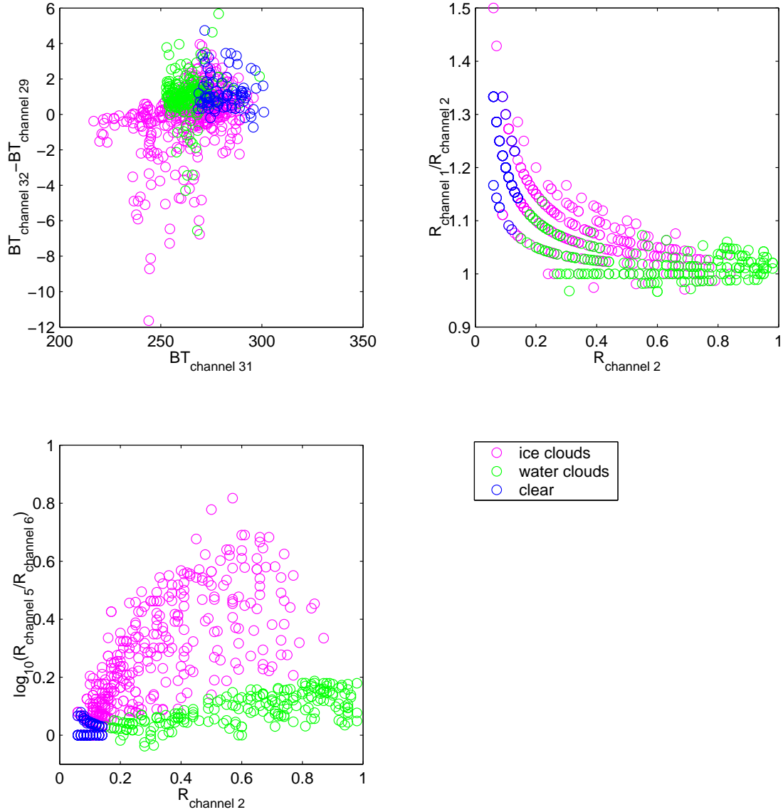
Figure 5: Scatterplots of BT_{channel_{31}} vs BT_{channel_{32}} - BT_{channel_{29}} (top left), R_{channel_1}/R_{channel_2} vs R_{channel_2} (top right), and R_{channel_2} vs \log_{10}(R_{channel_5}/R_{channel_6}) (bottom left).
