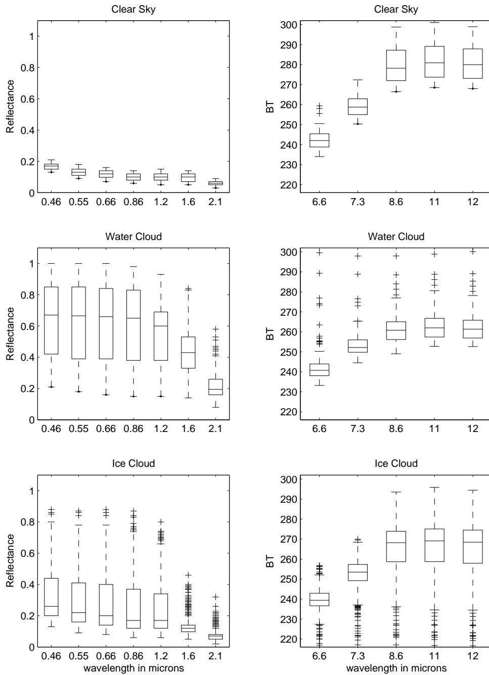
Figure 4: The boxplots of 7 reflectances and 5 brightness temperatures for clear sky, water clouds, and ice clouds over the ocean.
