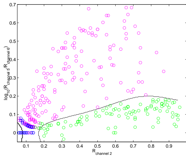
Figure 7: The classification boundaries determined by the nonstandard MSVM when the cost of misclassifying clouds as clear is 1.5 times higher than other types of misclassifications.
