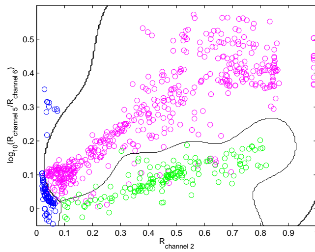
Figure 11: Classification boundaries on the training set based on the MSVM trained on two variables only.
