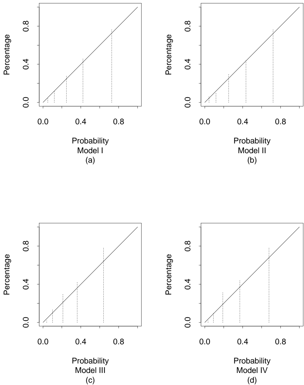
Figure 5.6: Estimates of Observed Fraction of 1's vs Expected Fraction, by Quintile, PSA models.
