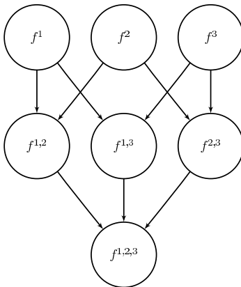
Figure 2: Hierarchical lattice for penalty
