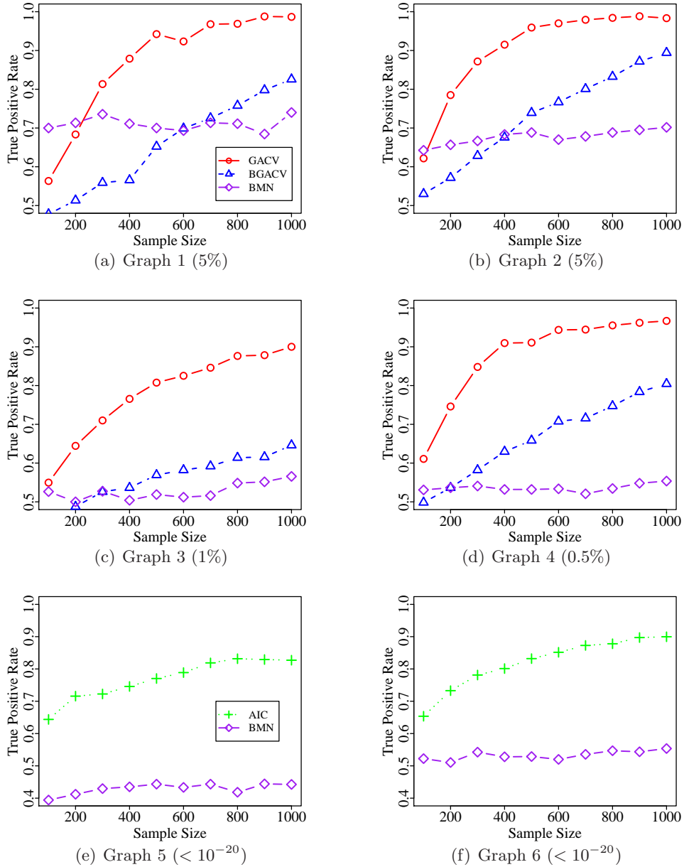
Figure 3: The True Positive Rate (TPR) of graph structure learning with increasing sample size by different methods. The percentage in the bracket is the upper bound of False Positive Rate (FPR) in each experiment. BMN always has larger FPR compared to GACV/BGACV/AIC.
