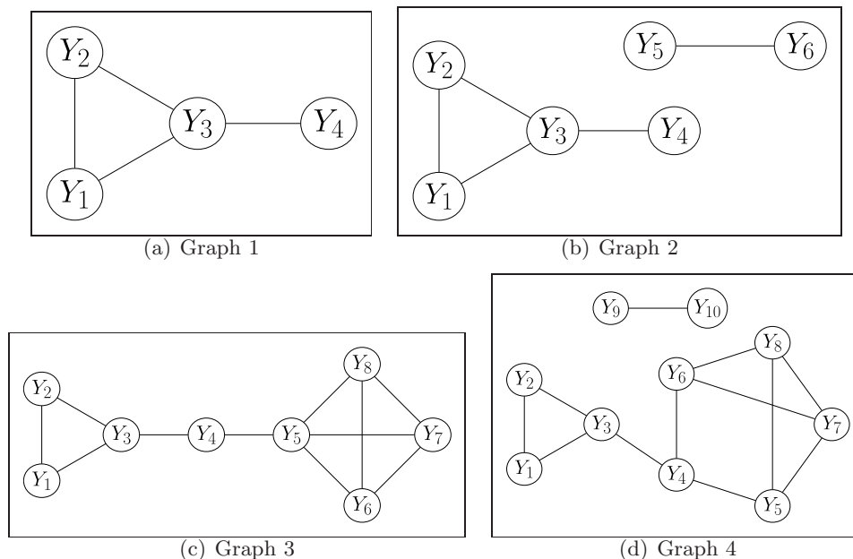
Figure 1: Graphical model examples.
