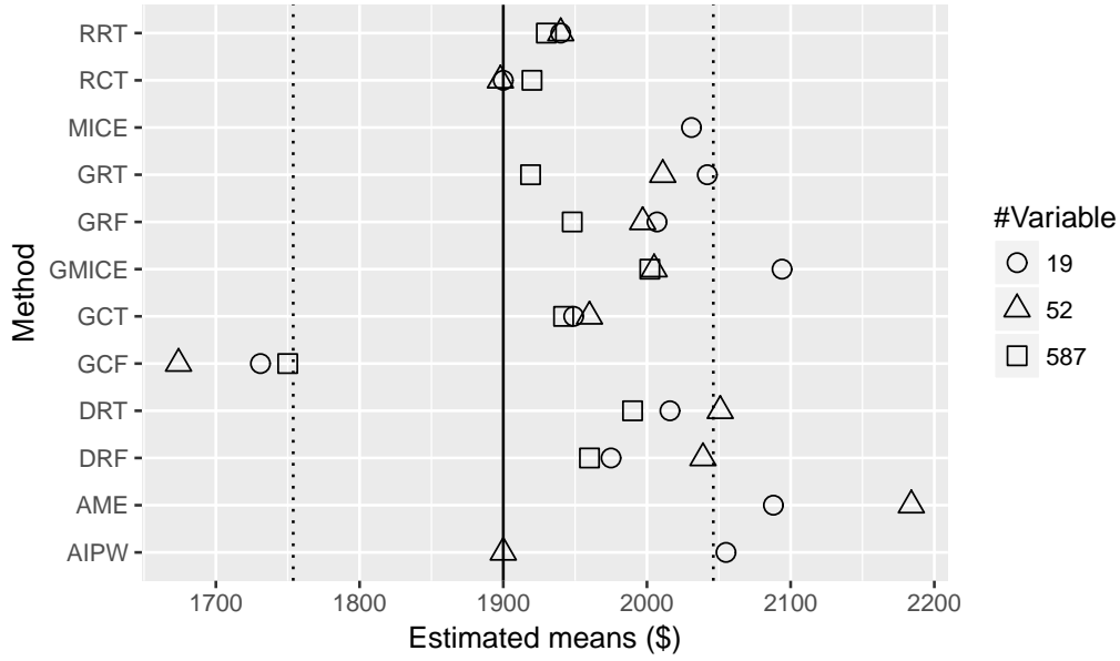
Figure 3: Estimates of mean INTRDVX (weighted by FINLWT21) for 2013 CE data using 19, 52 and 587 predictor variables. The solid line marks the value of the SIM estimate of $1900 and the dotted lines mark SIM plus and minus one standard error of $146 (calculated from balanced repeated replication weights).
