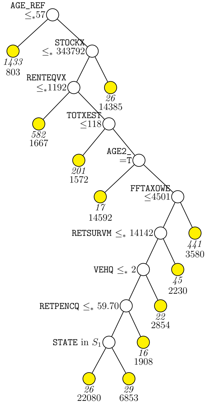
Figure 2: GUIDE regression tree for predicting INTRDVX. At each split, an observation goes to the left branch if and only if the condition is satisfied. The symbol ‘ \leq_* ’ stands for ‘ \leq or missing’. For splits on categorical variables, values not present in the training sample go to the right. Set S_1 = \{12, 13, 17, 29, 36, 48, 53, 6, 8, NA\} . Sample size ( in italics ) and mean of INTRDVX printed below nodes.
